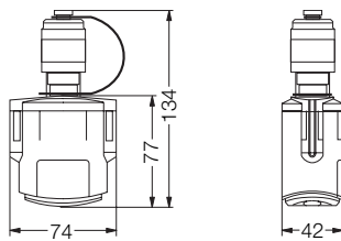
Y-Junction box
