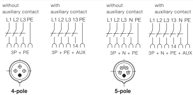
Plug 4/5-pole
