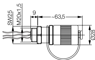
Receptacle metal version
