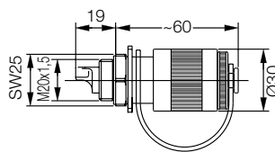
Inlet plastic version
