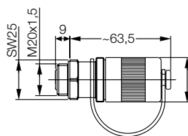
Receptacle plastic version
