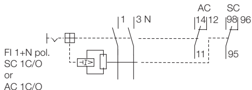
4-pole + AC or SC
