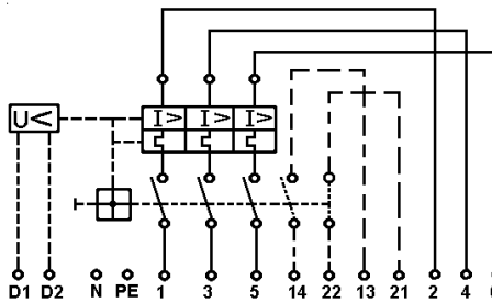
Contact arrangement - Manual motor starter
