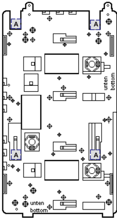
A = fixing point for manual motor starter
