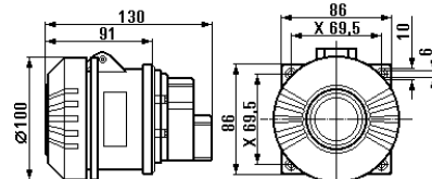
Flange socket, 5-pole
