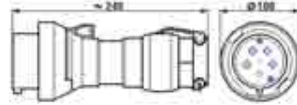
Plug, 5-pole
