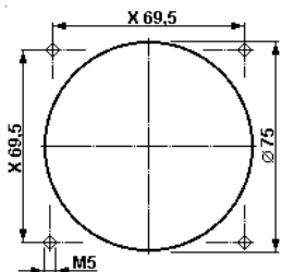
Drilling template for inlets
