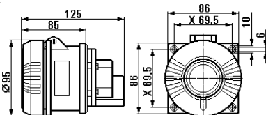
Flange socket, 3- and 4-pole
