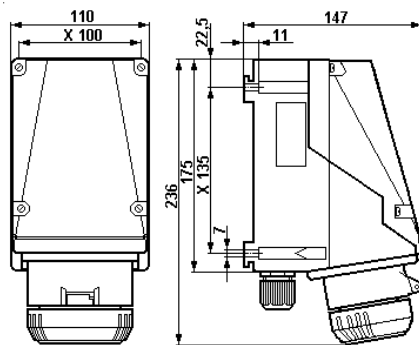
Wall socket 4-pole and 5-pole
