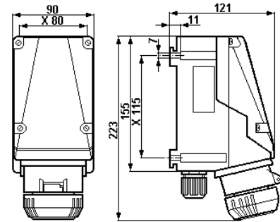
Wall socket 3-pole
