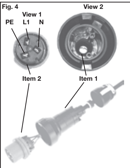
Fastening point A 16A socket 3-pol.
