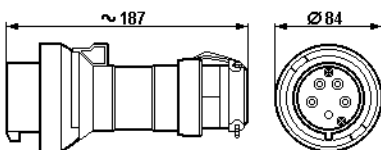
Plug 5-pole
