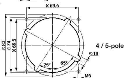
Drilling template for flange sockets
