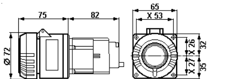
Flange socket 3-pole
