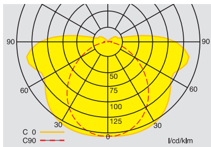
Polar curve SV EURO 4 with clear cover
