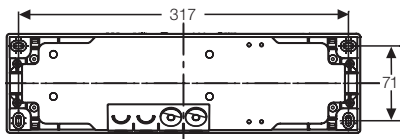
SV EURO 4 with cover PU
