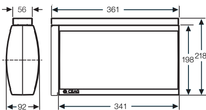
28021 LED CGLine with ceiling fastening
