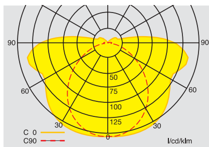
Polar curve 58011 with clear cover
