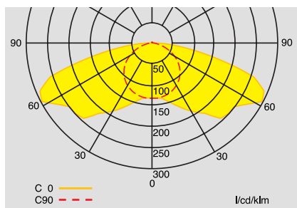
Polar curve 28011 with clear cover
