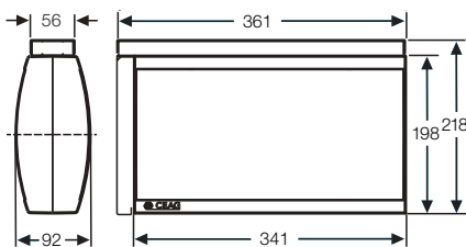
28021 with ceiling mounting
