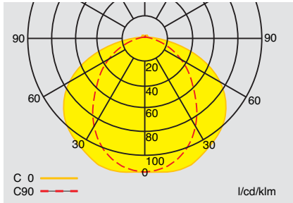
Polar curve 79011 CG-S
