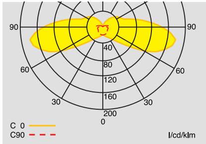
Polar curve 51011 CG-S with legend-cover
