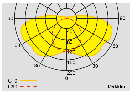
Polar curve 51011 CG-S with clear cover
