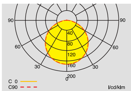
Polar curve 57011 CG-S with opaque cover
