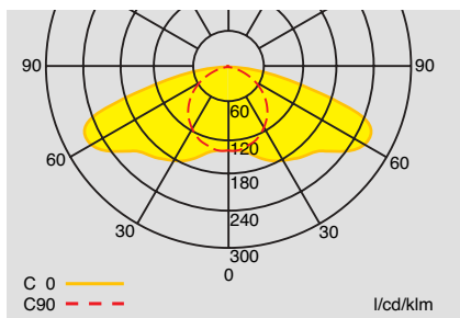
Polar curve 57011 CG-S with clear cover
