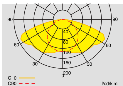
Polar curve 57011 CG-S with clear cover, silk screened structure
