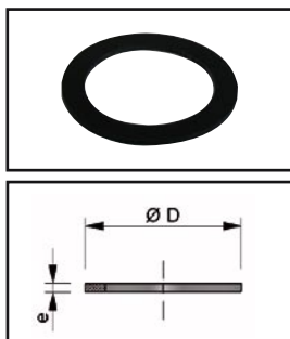
Joint plat Sealing washer
