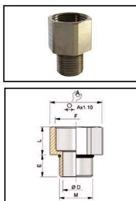
Amplificateur laiton nickelé Male/Femelle Adaptor nickel plated brass Male / Female
