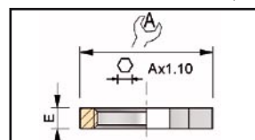
Ecrou / locknut
